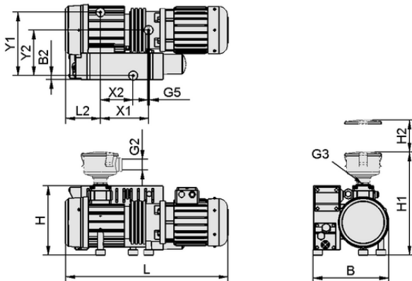
Design data EVE-OG 40 AC3
