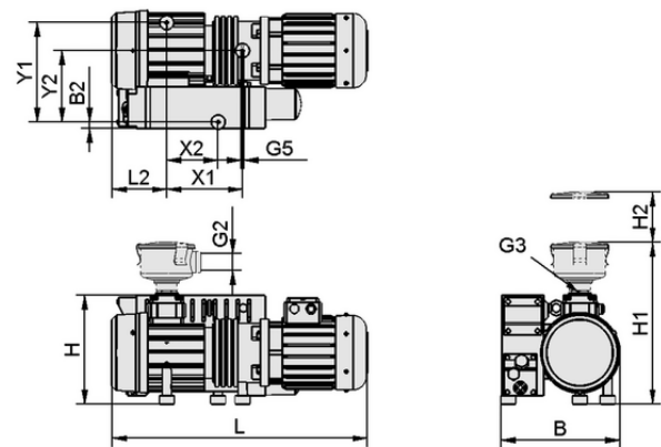
Design data EVE-OG 25 AC3 F
