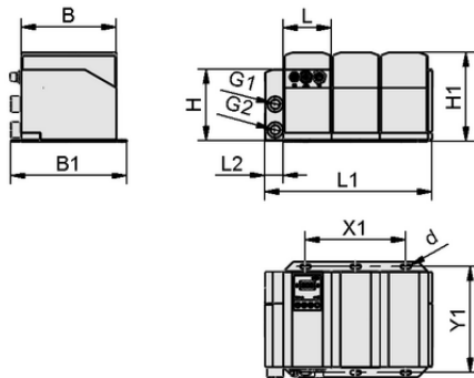
Design data GSPc 150 2xM12-5 24V-DC FB
