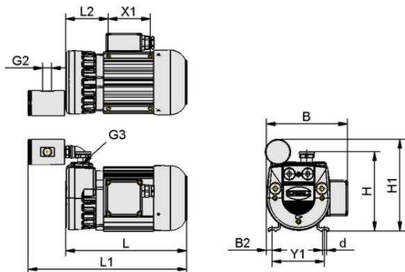
Design data EVE-TR 8 AC3 IE2-TYP1 F
