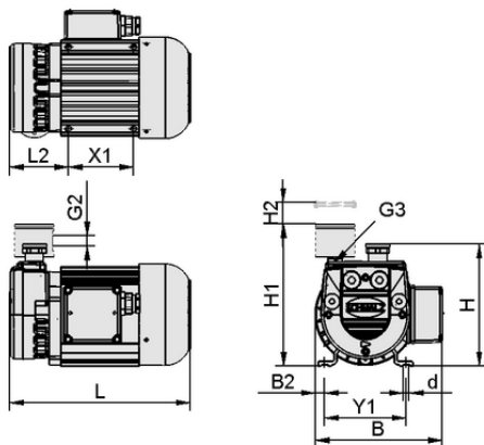
Design data EVE-TR 8 AC3 IE2-TYP1
