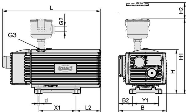
Design data EVE-TR 25 AC3 IE3-TYP4
