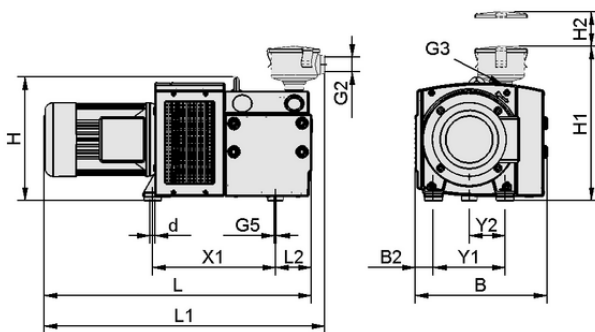
Design data EVE-TR 80 AC3 IE3-TYP4
