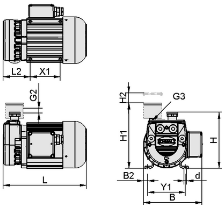
Design data EVE-TR 8 24V-DC F
