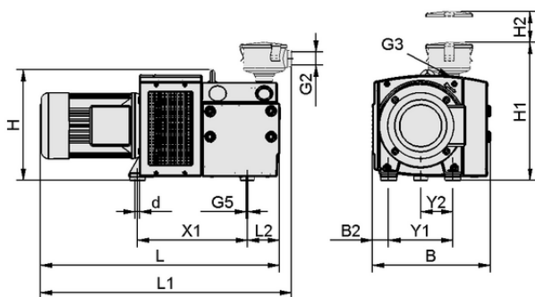
Design data EVE-TR 140 AC3 IE3-TYP3 VBV
