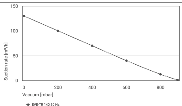
Suction rate at various degrees of evacuation
