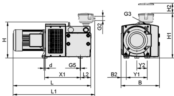
Design data EVE-TR 100 AC3 IE3-TYP3
