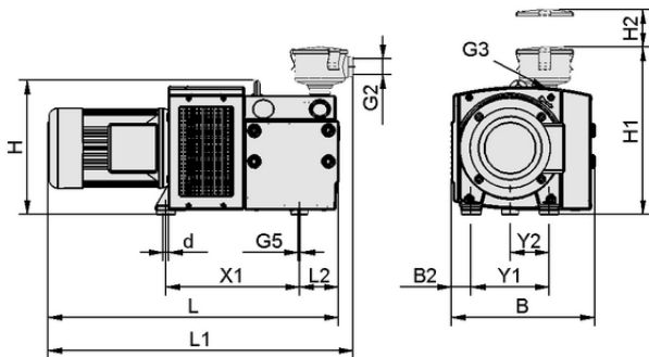
Design data EVE-TR 80 AC3 IE3-TYP3
