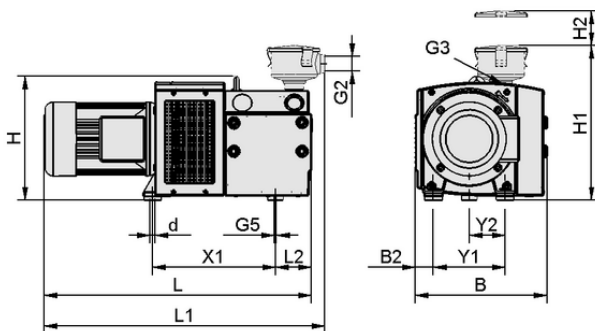
Design data EVE-TR 80 AC3 IE3-TYP1 F
