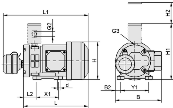
Design data EVE-TR 8 DC
