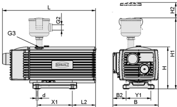
Design data EVE-TR-X 40 AC3 F-VB
