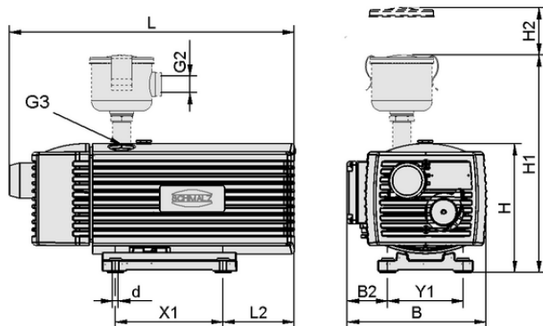
Design data EVE-TR-X 25 AC3 F-VB
