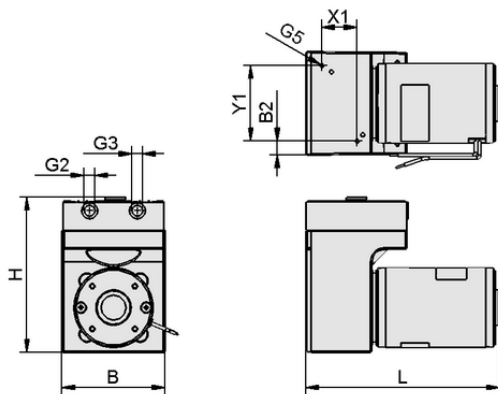
Design data EVE-TR-M 2.3 12V-DC
