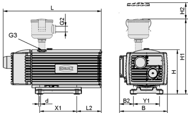
Design data EVE-TR 25 AC3 F
