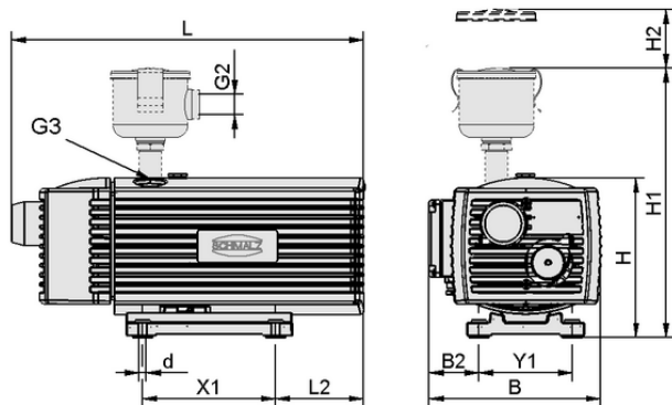
Design data EVE-TR 16 AC F
