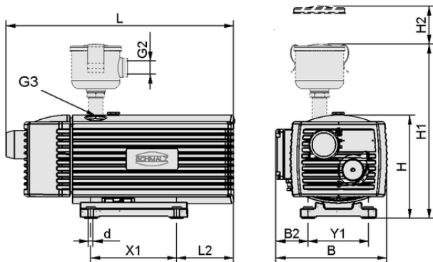
Design data EVE-TR 10 AC F
