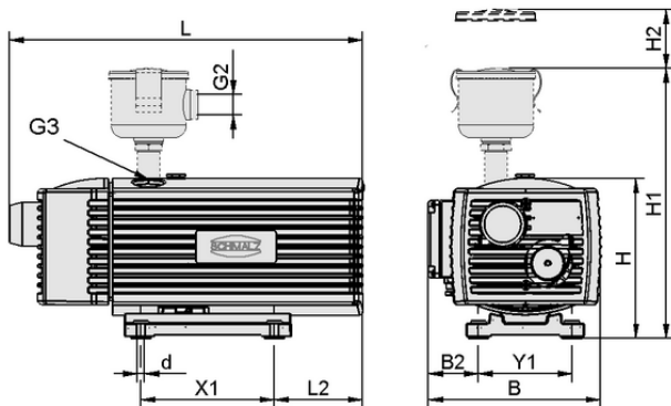
Design data EVE-TR 40 AC3
