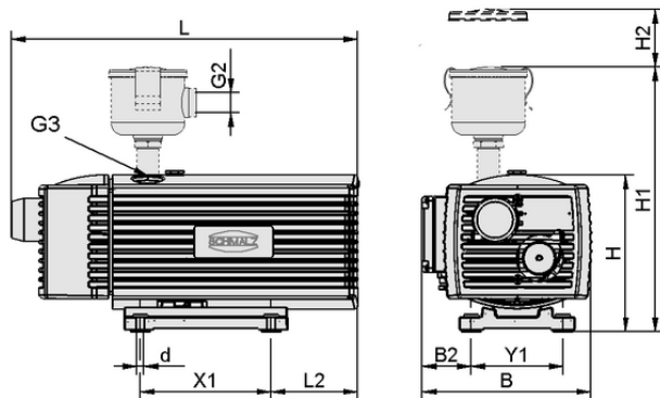
Design data EVE-TR 25 AC3
