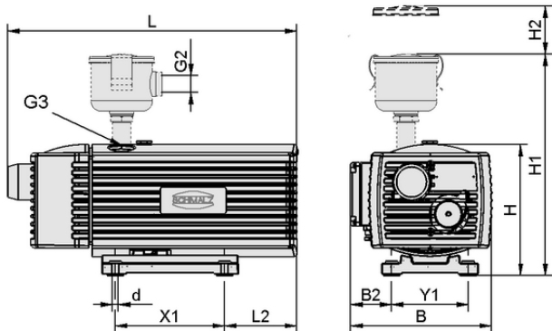
Design data EVE-TR 10 AC3
