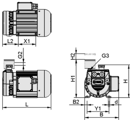
Design data EVE-TR 8 AC
