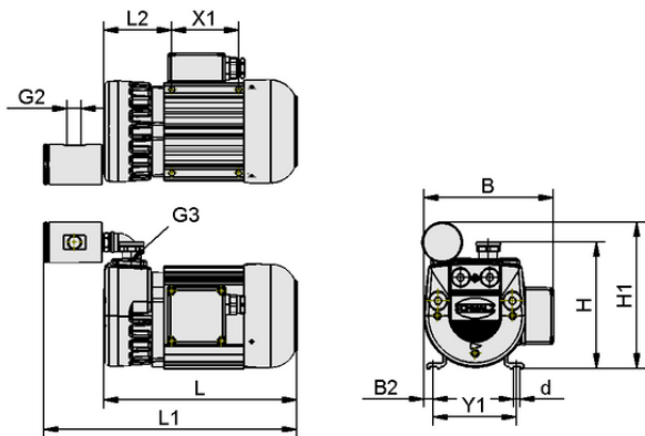
Design data EVE-TR 8 AC F
