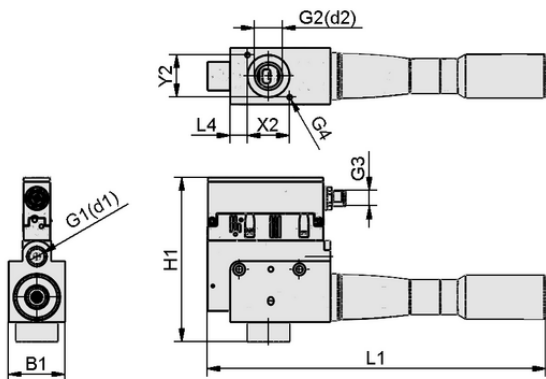
Design data SCPSc-L HV 3-16 NO M12-5 PNP
