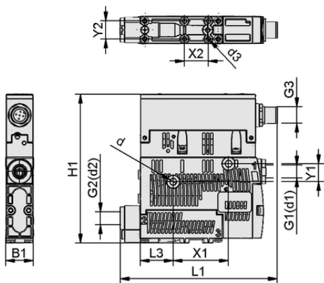
Design data SCPSc 07 G02 NO M12-5 PNP
