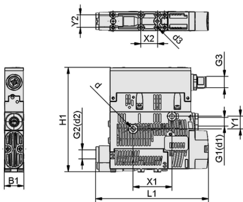
Design data SCPSc BY 2-14 G02 NC M12-5 NPN
