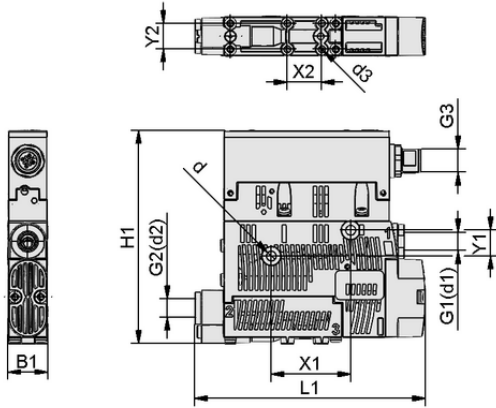
Tasarım verileri SCPSc BY 2-14 G02 NO M12-5 PNP
