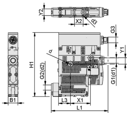
Design data SCPSi 10 M G02 IMP M12-5
