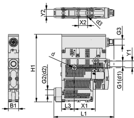
Design data SCPS 15 M G02 NO M12-5 PNP
