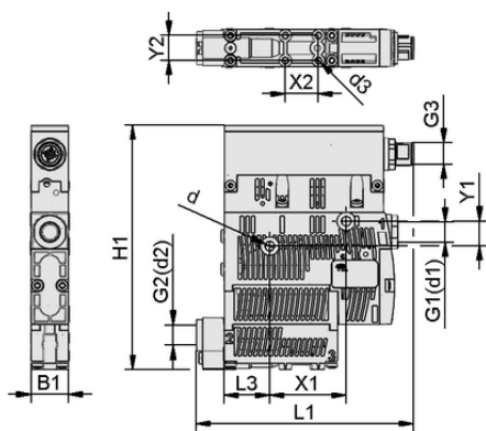
Design data SCPS 10 M G02 NO M12-5 PNP
