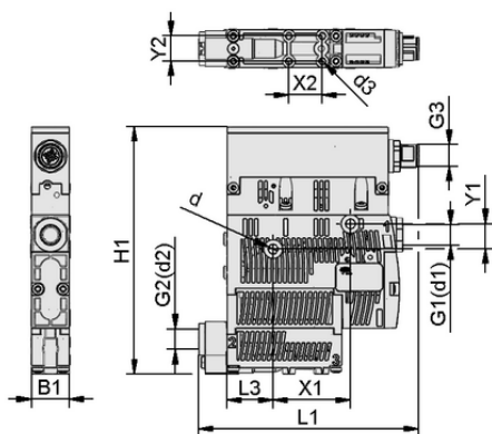
Design data SCPS 07 M G02 NO M12-5 PNP
