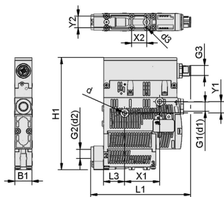
Design data SCPSi 07 M G02 NC M12-5
