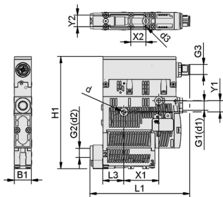
Design data SCPS 07 M G02 NC M12-5 PNP
