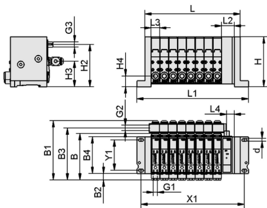
Design data SCTSi IOL 4
