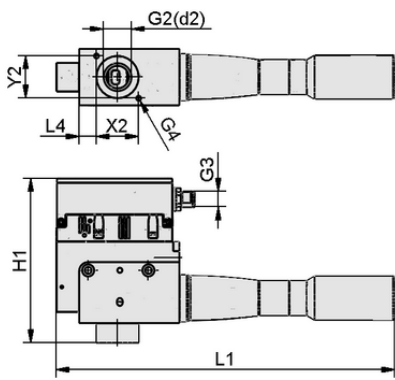
Design data SCPSi-L HV 3-20 NO M12-5
