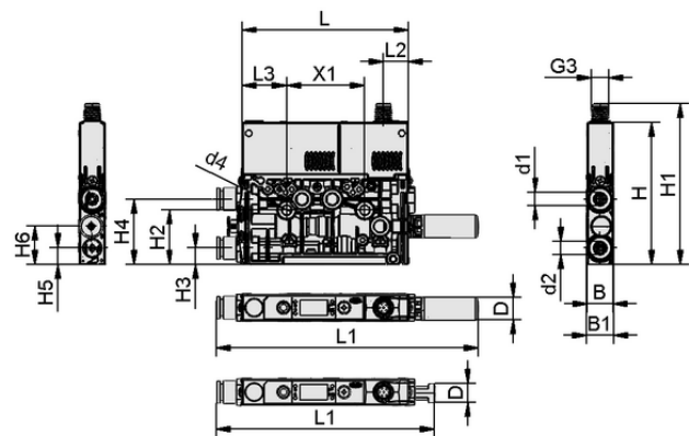
Design data SCPMc 07 S01 NO M8-6 PNP AAT
