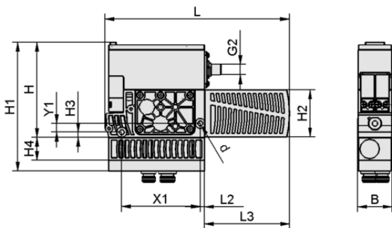
Design data SXMPi 25 IMP Q M12-5
