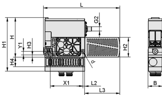
Design data SXMPi 25 IMP Q PC M12-5
