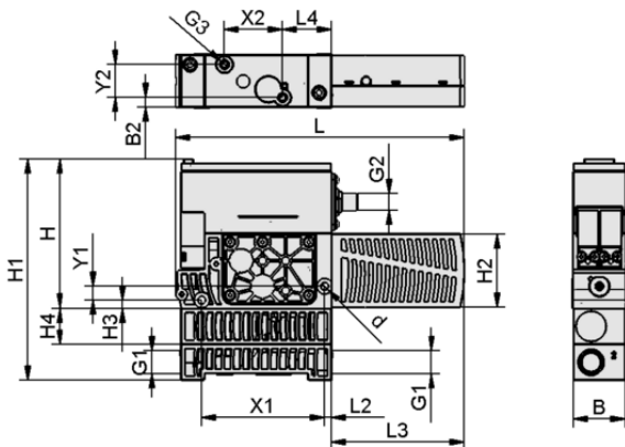
Design data SXMPi 25 IMP H PC M12-5
