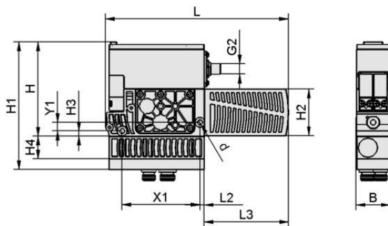
Design data SXMPi 30 NC Q PC M12-5
