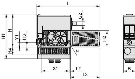
Design data SXMPi 25 NC Q M12-5
