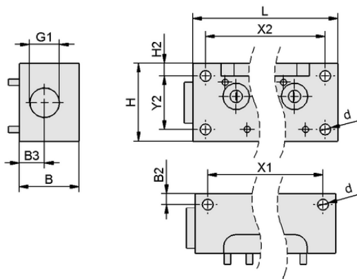
Design data GP 6 SCPS 07..15 G2
