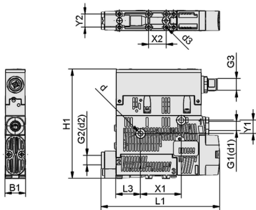
Design data SCPSi 2-14 G02 NO M12-5
