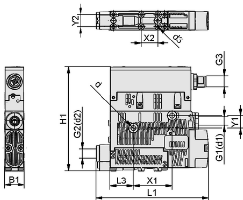
Design data SCPS 2-09 G02 NO M12-5 PNP
