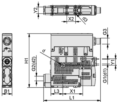
Design data SCPSi 15 G02 NC M12-5
