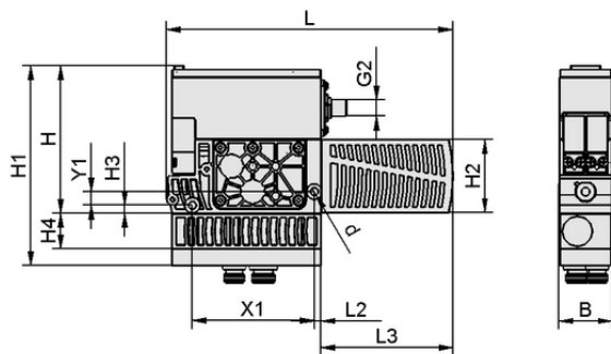
Design data SXMPi 30 NC Q 2xM12-5
