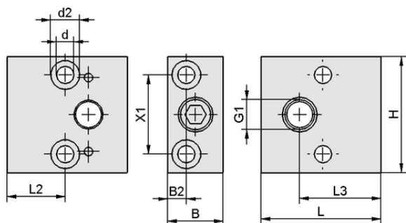
Design data ADP-EJ 45.5x21x44-G1/4-IG SEAC VA-L
