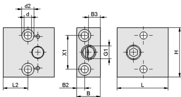
Design data ADP-EJ 45.5x21x44-G1/4-IG SEAC VA-S
