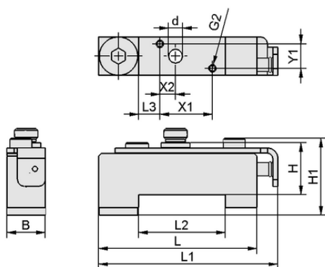
Design data ADP-Q 90.5x22x29.7 SMPi/SCPi
